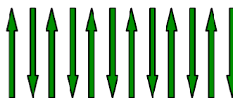
antiferromagnetism
