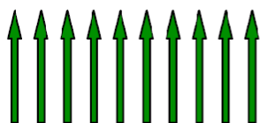
Ferromagnetism
