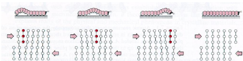
FIGURE 7.3 Representation of the analogy between caterpillar and dislocation motion.
