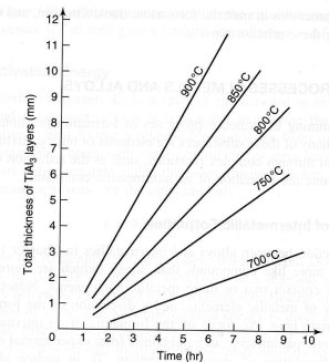
Figure 3.3 Rate of formation of TiAl_3 at various temperatures.
