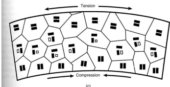
Figure 3.6 Shape-memory alloys transform from (a) a partially ordered, high-temperature austenitic phase to (b) a mixed austenite-martensite low-temperature state to (c) an ordered mid-phase state under deformation.
