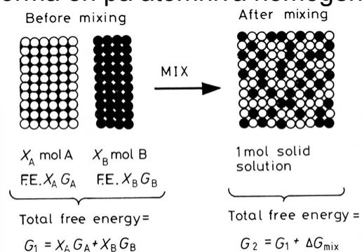
Fig. 1.7 Free energy of mixing.
