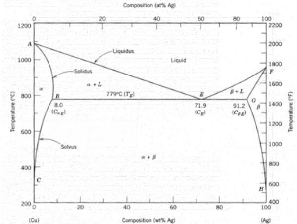
FIGURE 9.6 The copper-silver phase diagram. [Adapted from Binary Alloy
