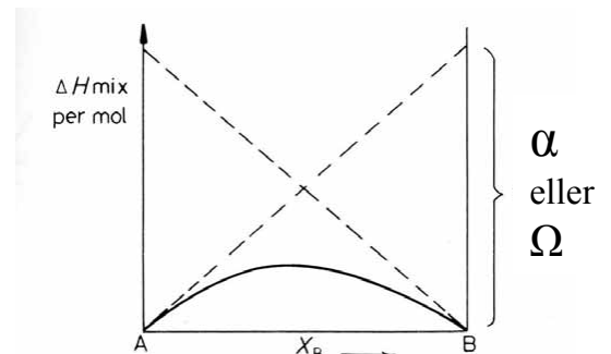
fig. 1.14 The variation of \Delta H_{mix} with composition for a regular solution.
