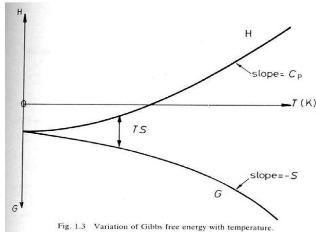
Fig. 1.3 Variation of Gibbs free energy with temperature.
