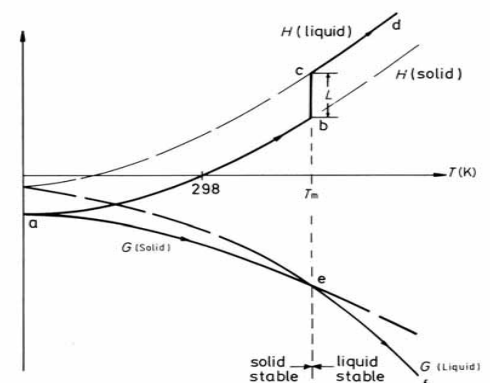
Fig. 1.4 Variation of enthalpy (H) and free energy (G) with temperature for the solid and liquid phases of a pure metal. L is the latent heat of melting. T_m the equilibrium melting temperature.
