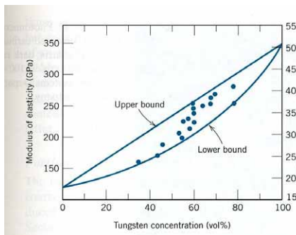
FIGURE 16.3 Modulus of elasticity versus volume percent tungsten for a composite of tungsten particles dispersed within a copper matrix. Upper and lower bounds are according to Equations 16.1 and 16.2; experimental data points are included. (From R. H. Krock, ASTM Proceedings , Vol. 63, 1963. Copyright ASTM, 1916 Race Street, Philadelphia, PA 19103. Reprinted with permission.)
