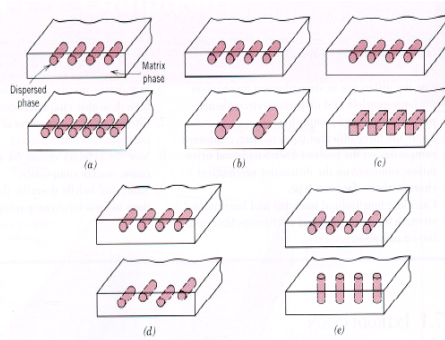
FIGURE 17.1 Schematic representations of the various geometrical and spatial characteristics of particles of the dispersed phase that may influence the properties of composites: (a) concentration, (b) size, (c) shape, (d) distribution, and (e) orientation. (From Richard A. Flinn and Paul K. Trojan, Engineering Materials and Their Applications , 4th edition, Copyright © 1990 by John Wiley & Sons, Inc. Adapted by permission of John Wiley & Sons, Inc.)
