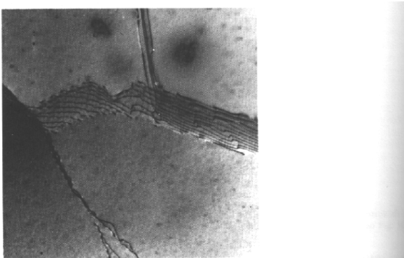
Figure 12 Electron micrograph of dislocation structures in low-angle grain boundaries in an Al-7 percent Mg solid solution. Notice the lines of small dots on the right. Mag. \times 17,000 . (R. Goodrich and C. Thomas.)
