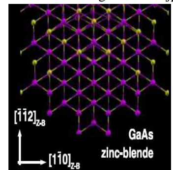
[Chrobak, Nowak, Nordlund, PRL 2006]
