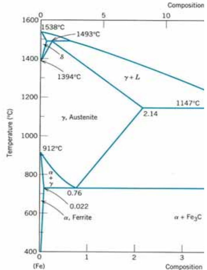
FIGURE 9.21 The iron-iron carbide phase diagram. Reprinted by permission of ASM International.
