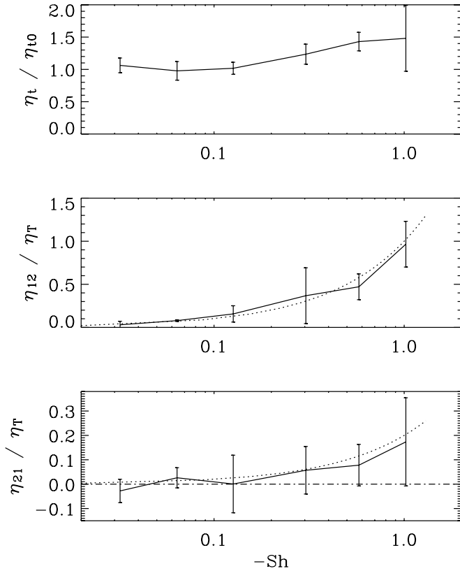
FIG. 3.—Dependence of \eta_t (normalized by \eta_{t0} ) as well as \eta_{12} and \eta_{21} (both normalized by \eta_T ) for homogeneous turbulence with shear on Sh for Re = 1.4 and Re_M = 14 . The dotted lines represent linear dependences on Sh .
