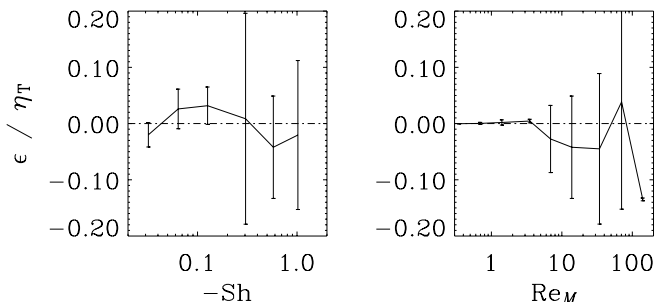
FIG. 6.— Dependences of \epsilon (normalized by \eta_T ) on \text{Sh} (left) and on \text{Re}_M (right) for the same runs as in Figs. 3 and 4, respectively.
