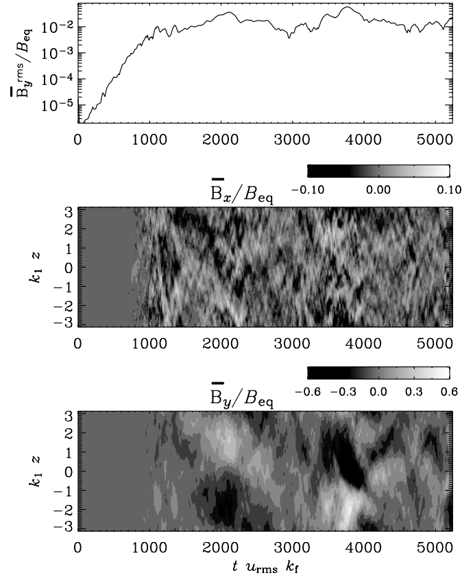
FIG. 7.— Time dependence of the rms value (with respect to z ) of \bar{B}_y (top) and spacetime diagrams \bar{B}_x(z, t) and \bar{B}_y(z, t) [all in units of B_{\text{eq}} , where B_{\text{eq}} = (\mu_0 \langle \rho u^2 \rangle)^{1/2} ] from a direct simulation with \text{Re}_M = 130 , \text{Pr}_M = 7 , k_f/k_1 = 10 , and \text{Sh} \approx -0.15 . The top panel demonstrates the initial exponential growth of the mean field (the growth rate is 0.009 u_{\text{rms}} k_f ). The other panels show episodes of large scales in z especially in the \bar{B}_y component. [See the electronic edition of the Journal for a color version of this figure.]
