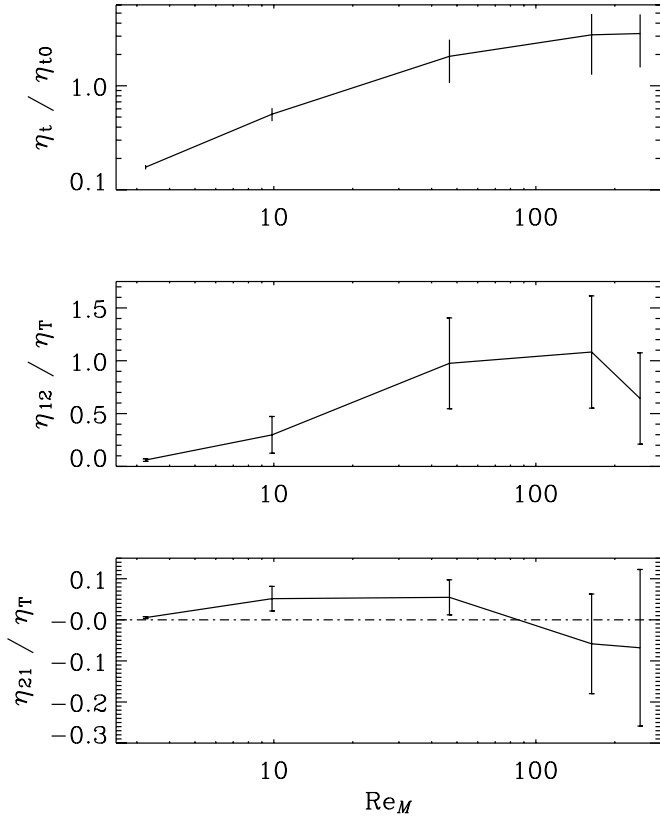
FIG. 5.— Same as Fig. 4, but for a fixed magnetic Prandtl number, \text{Pr}_M = 20 . Here, \text{Re} = \text{Re}_M/20 is not constant. Because u_{\text{rms}} increases with increasing \text{Re}_M , \text{Sh} is also not constant and varies between -2.5 (for \text{Re} = 0.16 ) and -0.3 (for \text{Re} = 13 ). Note that \eta_{21} turns negative at about \text{Re}_M = 100 . However, the errors are larger than the mean.
