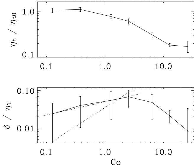
FIG. 1.—Dependence of the normalized \eta_t and \delta on Co for homogeneous turbulence with rotation for Re = 1.3 and Re_M = 13 . The vertical lines indicate error bars. Note that there is a maximum of \delta/\eta_T at Co \approx 3 . For Co < 3 the results for \delta/\eta_T are best described by \delta/\eta_T \approx 0.05Co^{0.35} , given by the dash-dotted line, but also a linear dependence, \delta/\eta_T \approx 0.035Co , indicated by the dotted line, is compatible within error bars.
