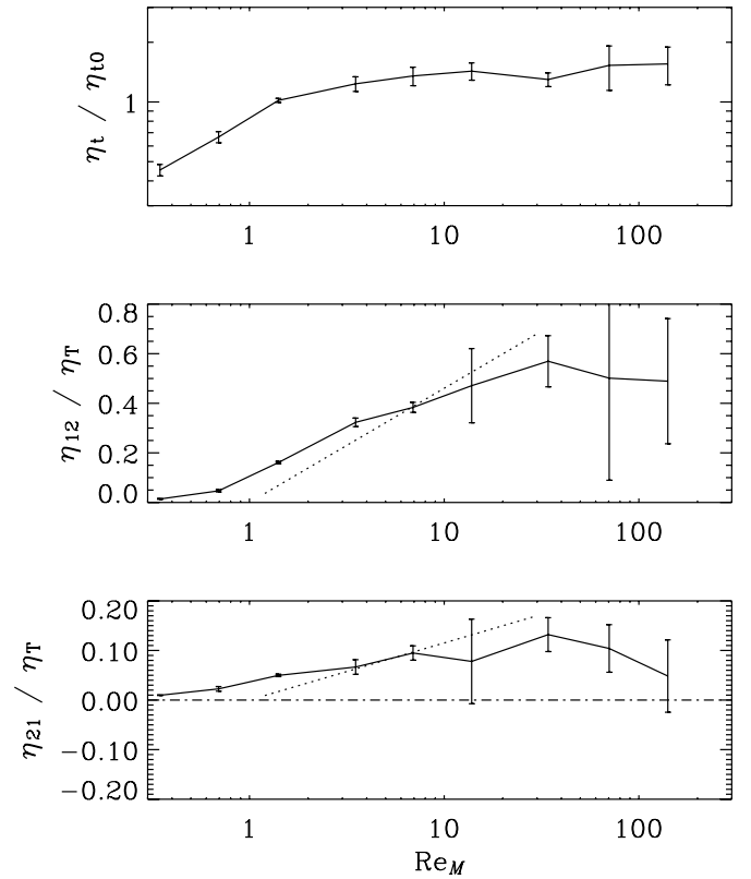
FIG. 4.—Dependences of \eta_t (normalized by \eta_{t0} ), as well as \eta_{12} and \eta_{21} (both normalized by \eta_T ) for homogeneous turbulence with shear on Re_M for Re = 1.4 and Sh = -0.6 . The dotted lines correspond to \eta_{12}/\eta_T = 0.2 \ln Re_M and \eta_{21}/\eta_T = 0.05 \ln Re_M and illustrate that \eta_{12}/\eta_T and \eta_{21}/\eta_T vary only weakly with Re_M .
