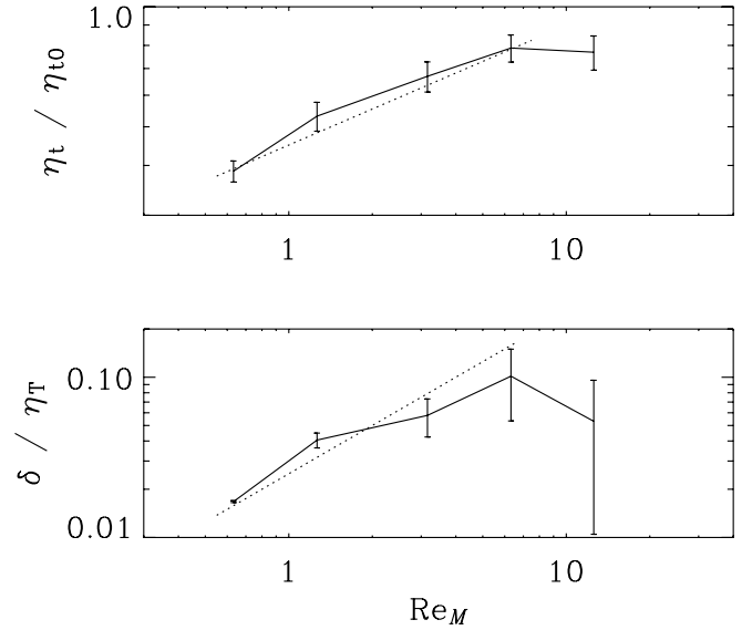
FIG. 2.—Dependence of the normalized \eta_t and \delta on Re_M for homogeneous turbulence with rotation for Re = 1.3 and Co = 1.3 . The dotted lines show the power-law fits \eta_t/\eta_{t0} = 0.45Re_M^{0.3} and \delta/\eta_T = 0.025Re_M which apply for Re_M < 7 .
