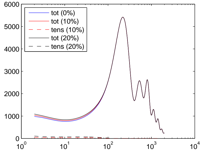
Temperature ( C_l^{TT} )
