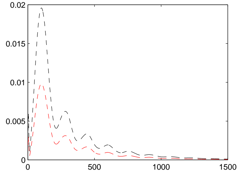
E-mode polarization ( C_l^{EE} )
