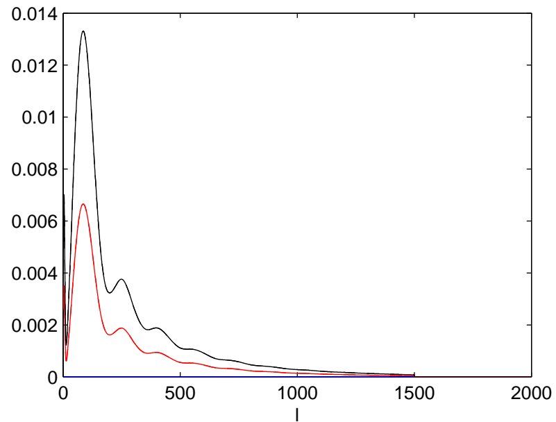
B-mode polarization ( C_l^{BB} )
