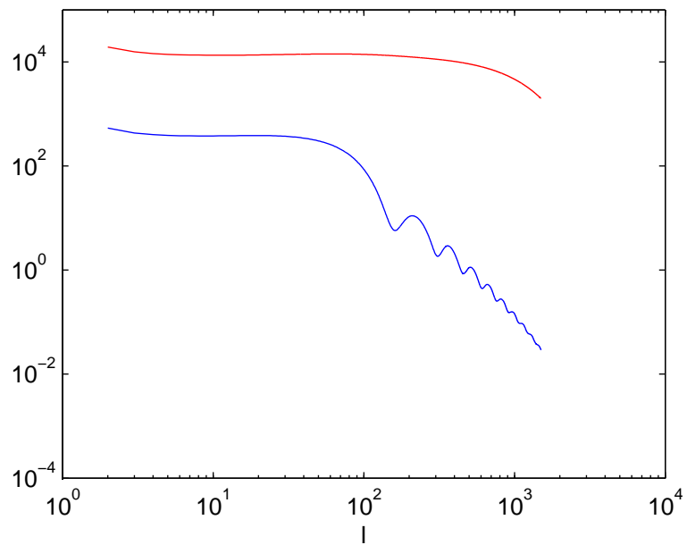
Temperature C_l^{TT}
