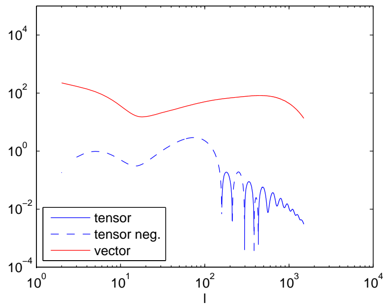
Cross correlation C_l^{TE}
