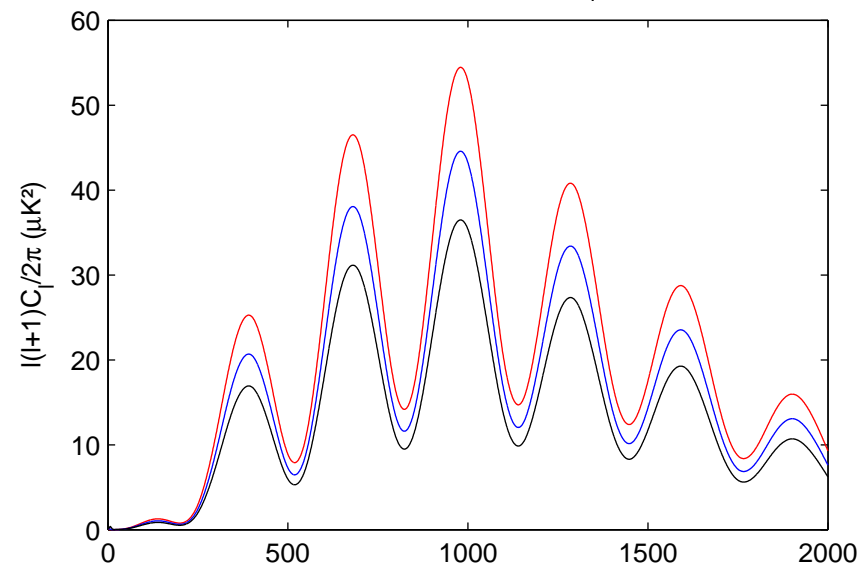
E-mode polarization ( C_l^{EE} )
