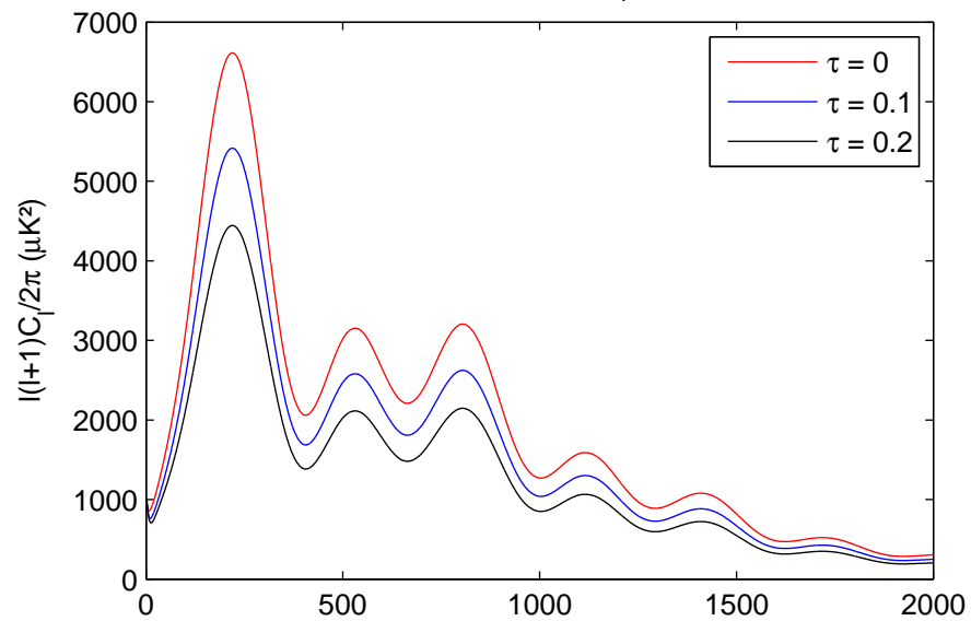
Temperature ( C_l^{TT} )
