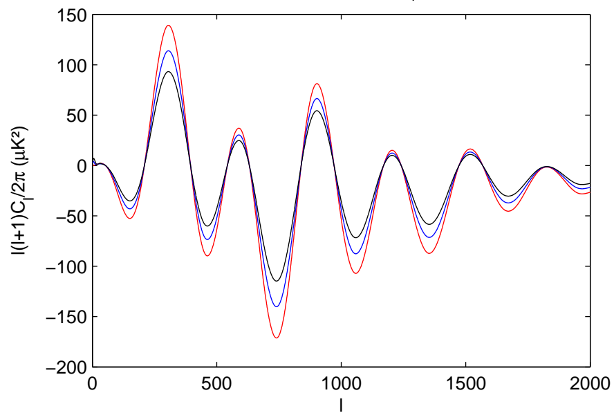
Cross correlation ( C_l^{TE} )
