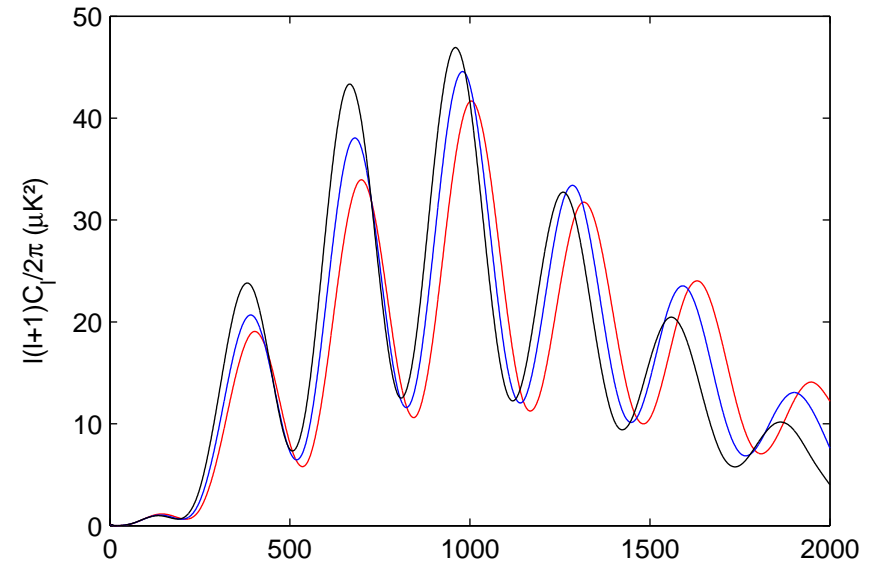
E-mode polarization ( C_l^{EE} )
