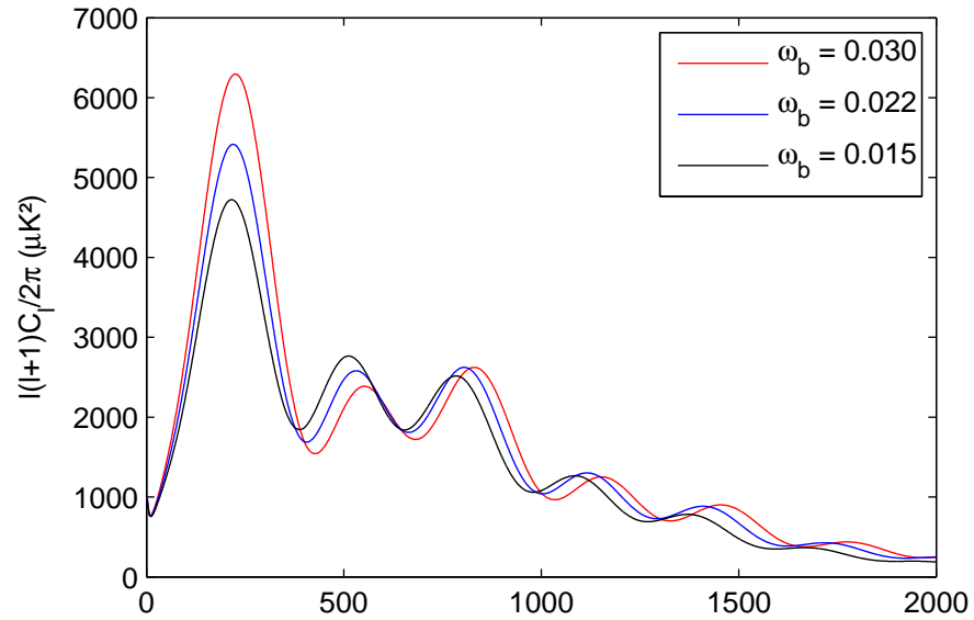
Temperature ( C_l^{TT} )
