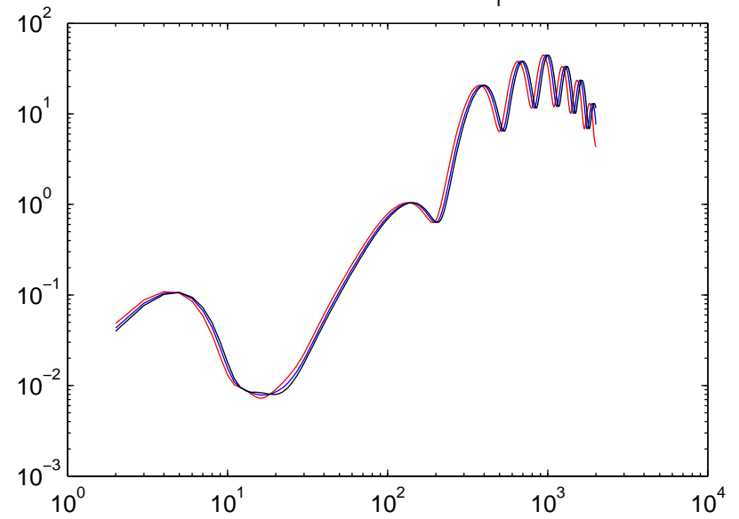
E-mode polarization ( C_l^{EE} )
