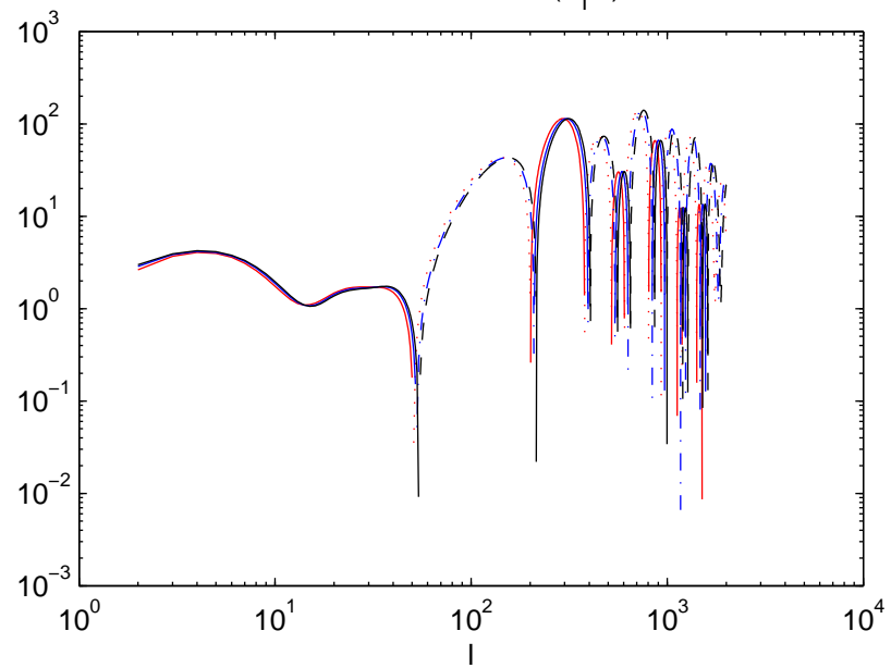
Cross correlation ( C_l^{TE} )
