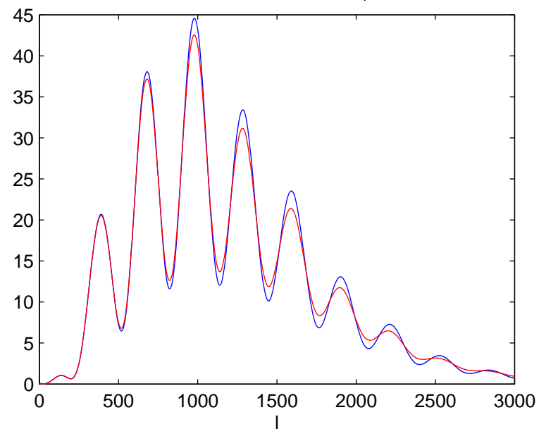
E-mode polarization C_l^{EE}
