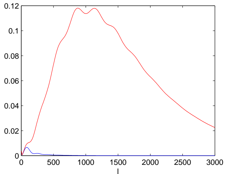
B-mode polarization C_l^{BB}
