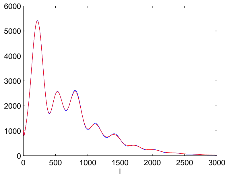
Temperature C_l^{TT}
