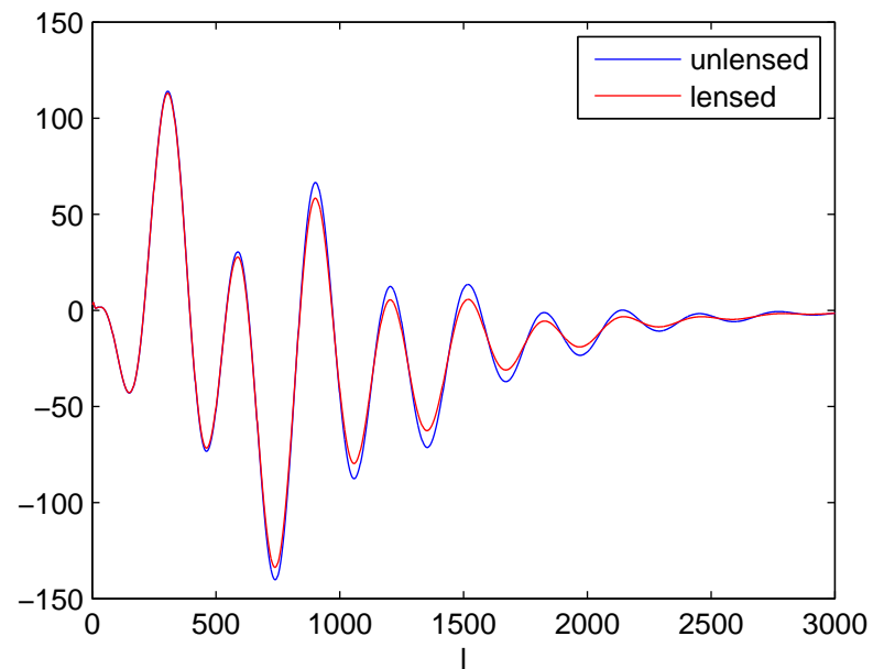
Cross correlation C_l^{TE}
